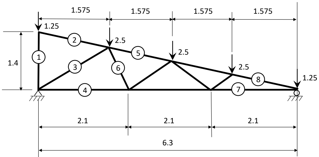
Analysis model
