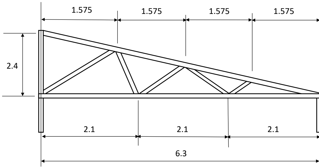
Engineering model
